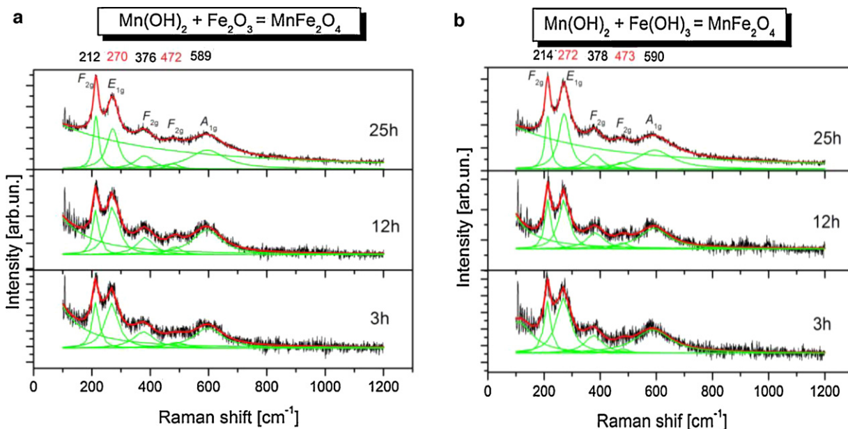
Fig. 2. Raman spectra at room temperature of the mixture of: (a) \text{Mn}(\text{OH})_2 and \alpha\text{-Fe}_2\text{O}_3 and (b) \text{Mn}(\text{OH})_2 and \text{Fe}(\text{OH})_3 powders after various milling time.
