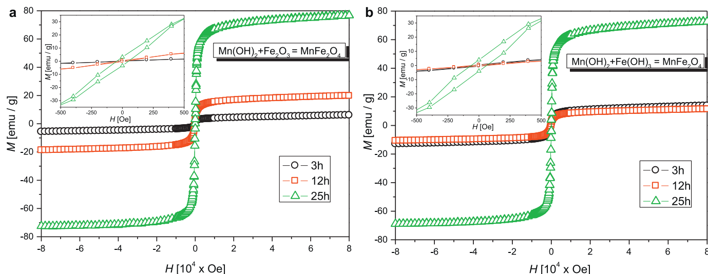
Fig. 7. The magnetic hysteresis curves of the mixture of: (a) \text{Mn}(\text{OH})_2 and \alpha\text{-Fe}_2\text{O}_3 and (b) \text{Mn}(\text{OH})_2 and \text{Fe}(\text{OH})_3 powders after various milling time. The inset shows low magnetization behavior.
