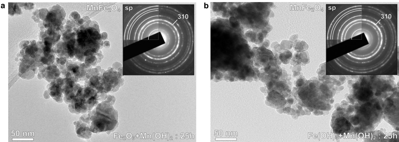
Fig. 5. TEM image with corresponding EDP of (a) Mn(OH) 2 and α-Fe 2 O 3 and (b) Mn(OH) 2 and Fe(OH) 3 after milling for 25 h. Spinel-type reflections dominate the diffraction pattern ( inset ).
