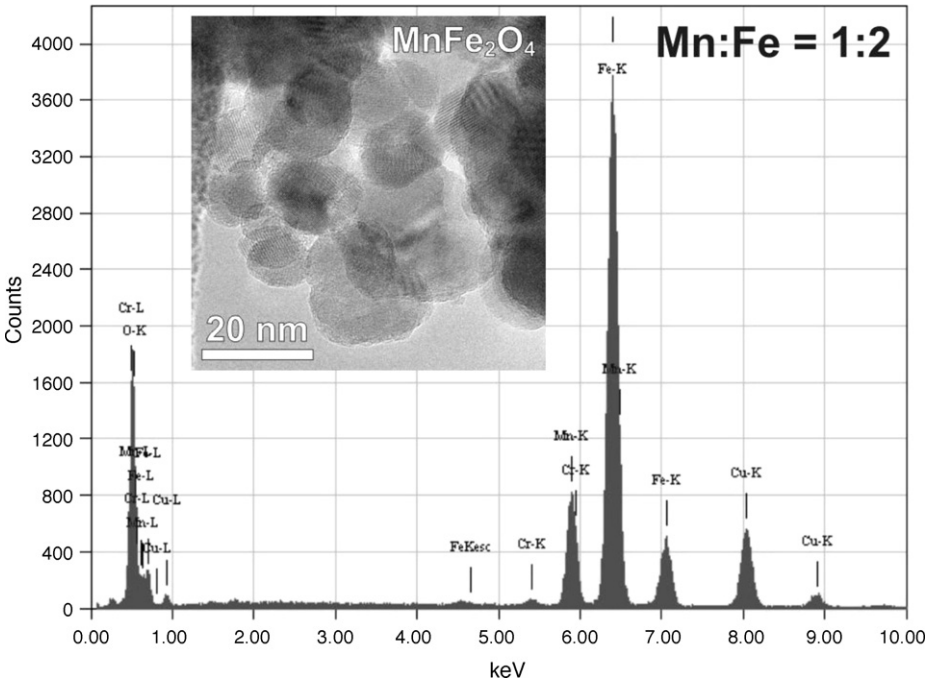
Fig. 6. EDS spectrum of Mn(OH) 2 and α-Fe 2 O 3 after milling for 25 h shows the presence of single MnFe 2 O 4 phase. The inset shows a HRTEM image of rounded MnFe 2 O 4 nanoparticles with well resolved lattice fringes, characteristic for the spinel structure. Cu peak stems from the Cu-grid of the TEM specimen, whereas the minor peak of Cr could not be explained.
