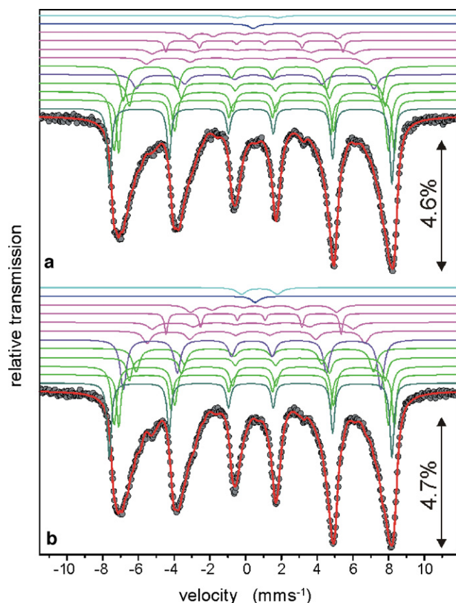
Fig. 8. Mössbauer spectra at room temperature of the mixture of: (a) \text{Mn(OH)}_2 and \alpha\text{-Fe}_2\text{O}_3 and (b) \text{Mn(OH)}_2 and \text{Fe(OH)}_3 powders after 25 h milling time.
