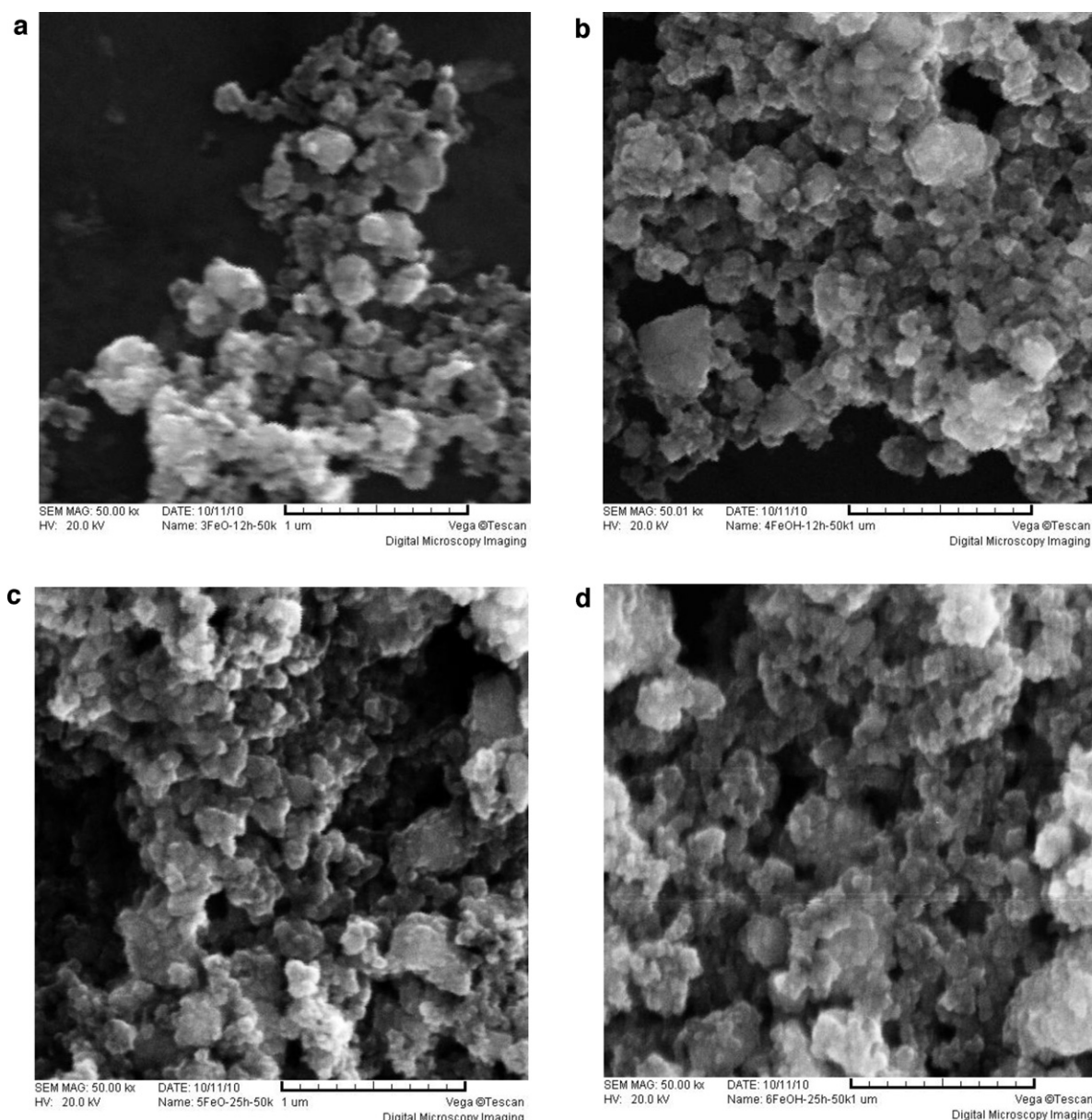
Fig. 4. SEM images of nanoscale mechanosynthesized of \text{MnFe}_2\text{O}_4 after 12 h and 25 h of milling of the mixture of: (a) \text{Mn}(\text{OH})_2 and \alpha\text{-Fe}_2\text{O}_3 and (b) \text{Mn}(\text{OH})_2 and \text{Fe}(\text{OH})_3 powders, respectively.
